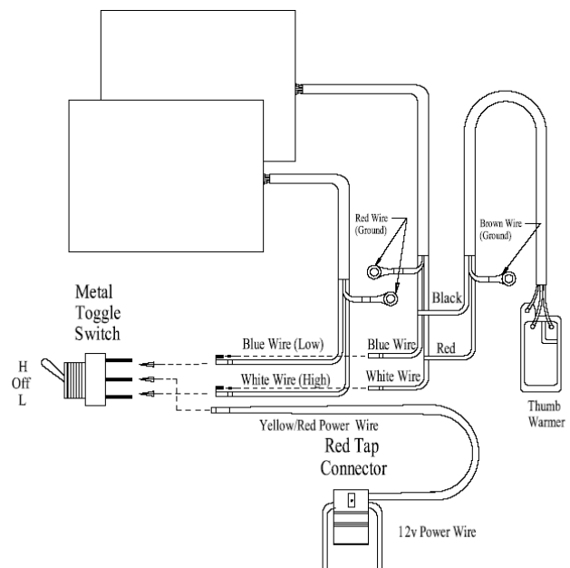
Figure 4. Hand Warmer w/210010 Type Thumb Warmer.
