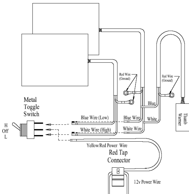
Figure 3. Hand Warmer w/210008 Type Thumb Warmer.
